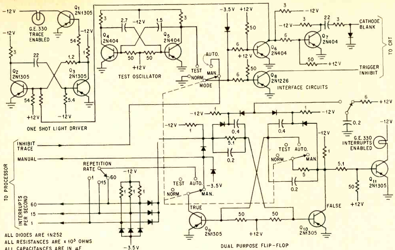
Oscilloscope modifications required for Strobes. These circuits are mounted on a circuit board housed in the preamplifier storage bay on the oscilloscope cart; only the two leads at the upper right are connected to the oscilloscope itself.
