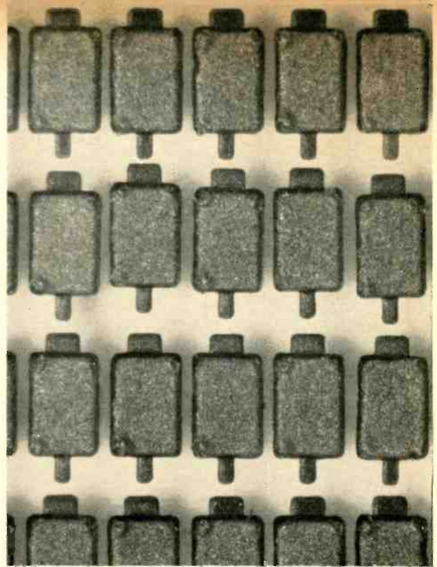
Diodes viewed from the bottom after separation. Each silicon chip measures 14 by 20 mils. For forward conduction, positive bias is applied to smaller terminals.
