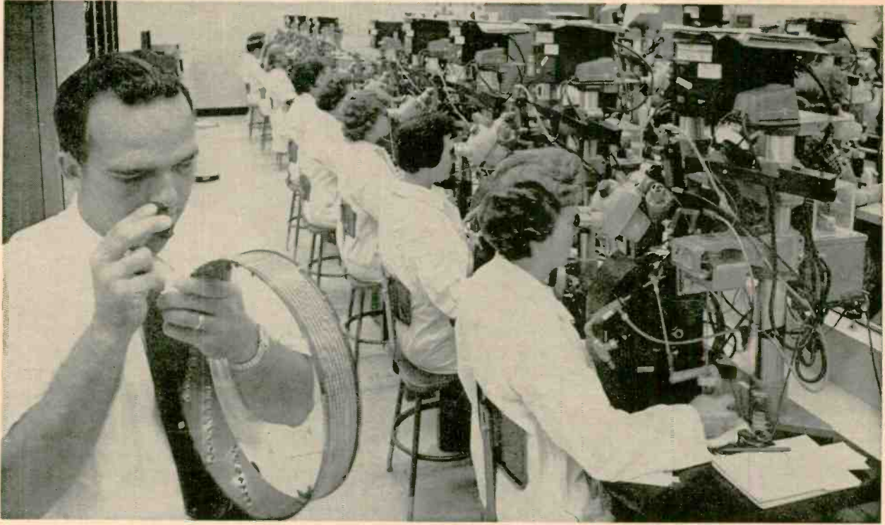
Drumfull of transistors is given a spot check (left) after lead bonding. The lead-bonding machines are at right.
