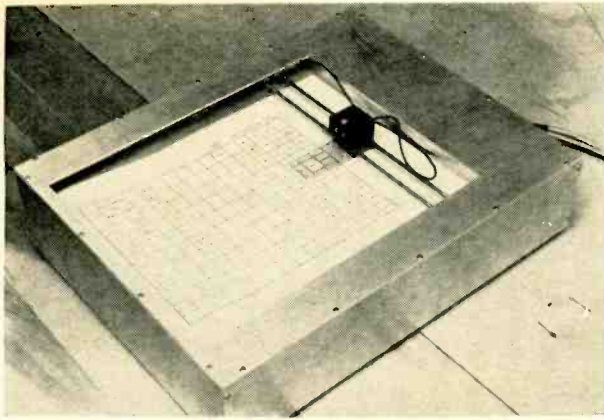
Prototype Datacoder terminal used with a teletypewriter for quick and accurate input of repetitive data. Data is selected by placing the little window over the appropriate square and pressing the button on the slider. This transmits two Teletype characters that give the location of the window, thus indicating the item specified.
