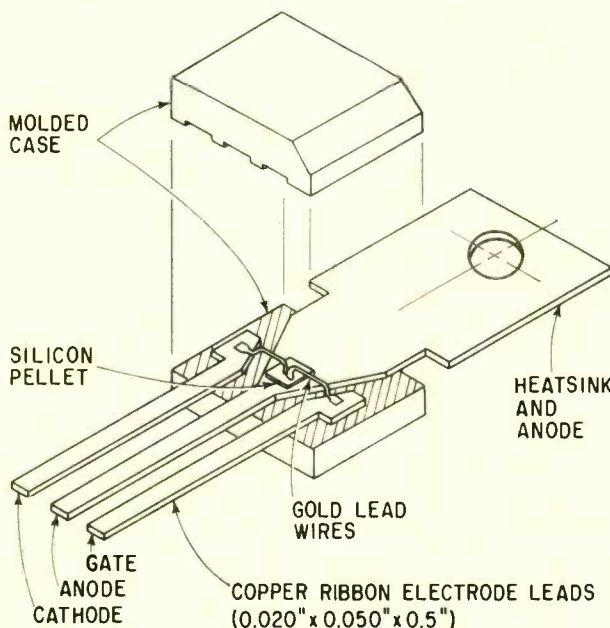
Package design for a silicon controlled rectifier. Sketch shows how chip is mounted on leads and encapsulated. Leads are preformed in copper strip, then sheared to cut the scr free after encapsulation. Over-all length of this scr is 1.3 inches. GE calls the chip a pellet.
