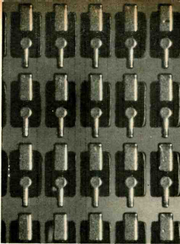
Each diode on this wafer—seen from above—weighs 100 micrograms. Diodes are manufactured by a batch process; assembly in equipment is readily automated.
